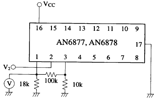
Test Circuit 6 (I Bias2 , I Bias3 )
