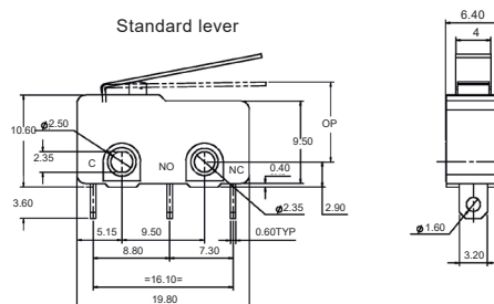
Standard lever
