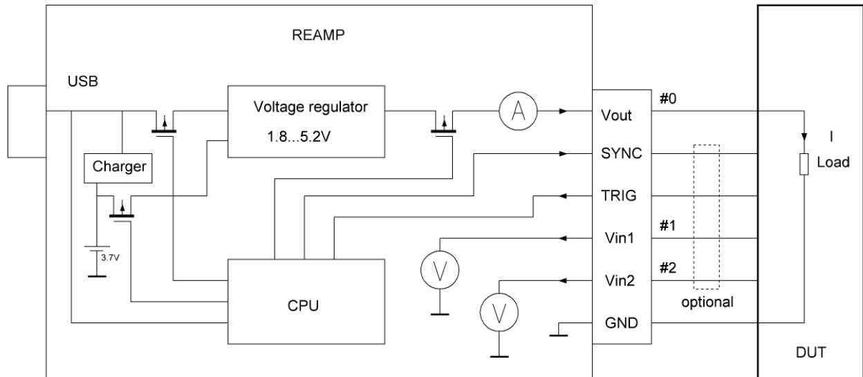
Fig. 2.1. Functional and connection diagram
