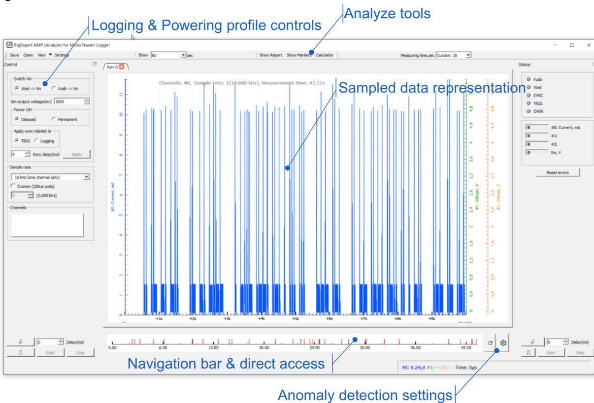
Fig. 3.2. Main window
